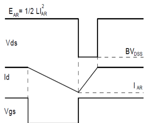
Fig.3-2 Avalanche waveform
