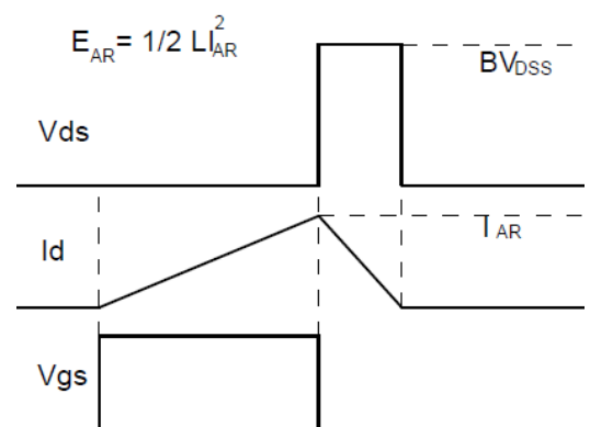
Fig.3-2 Avalanche waveform
