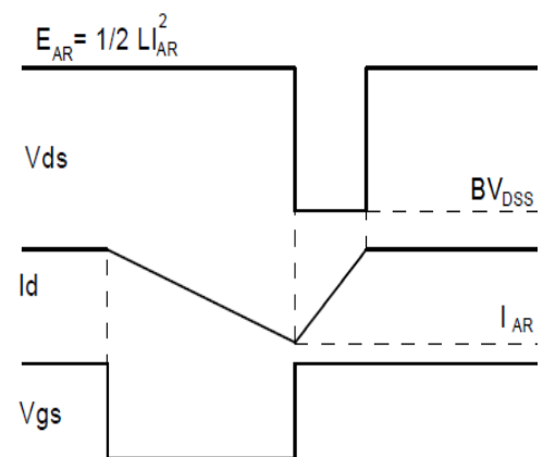
Fig.3-2 Avalanche waveform
