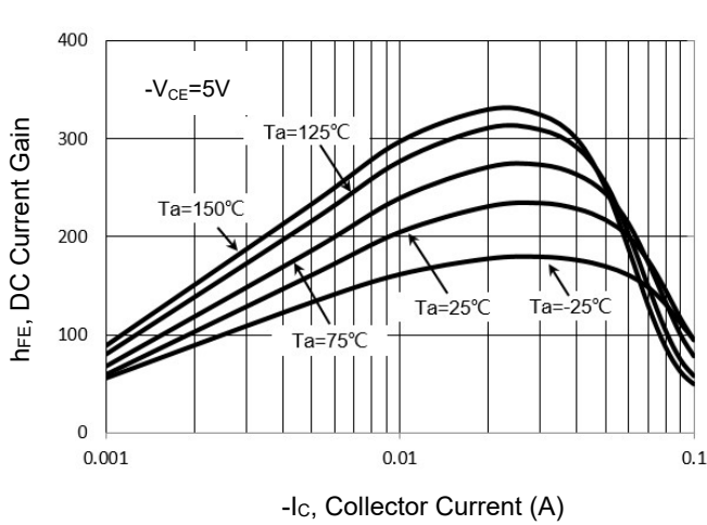
Fig 3. DC Current Gain vs. Collector Current
