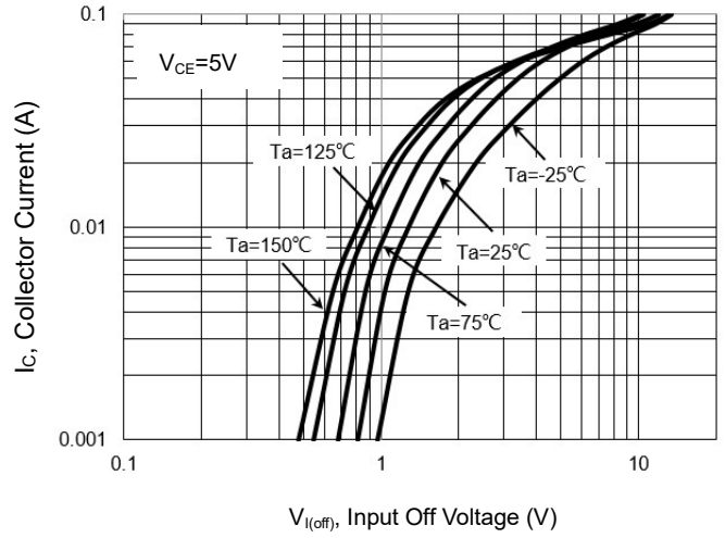
Fig 2. V_{I(off)} vs. Collector Current
