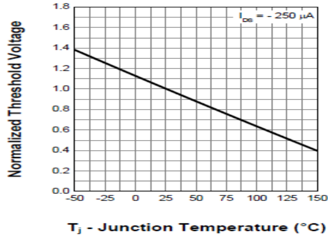
Fig. 2 Gate Threshold Variation vs. T_j
