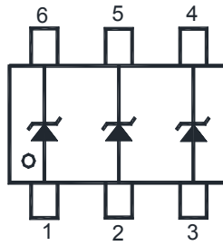
1. Anode 2. Anode 3. Anode 4. Cathode 5. Cathode 6. Cathode SOT-363 Plastic package
