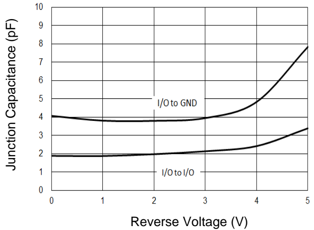
Fig 4. Junction Capacitance
