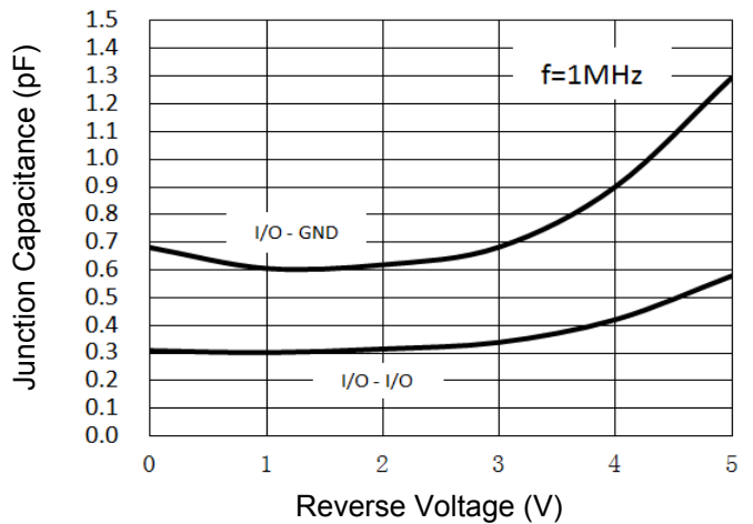
Fig 4. Junction Capacitance
