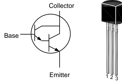
1. Collector 2. Base 3. Emitter TO-92 Plastic Package
