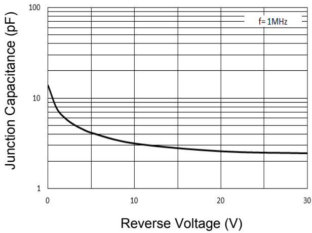
Fig 3. Junction Capacitance
