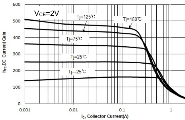
Fig. 3 h_{FE,DC} Current Gain vs. Collector Current
