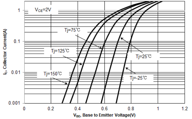
Fig. 2 Collector Current vs. Base-Emitter Voltage
