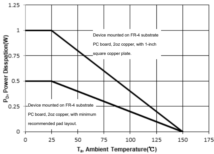
Fig. 7 Power Derating Curve
