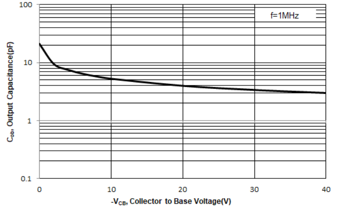
Fig. 6 Junction Capacitance
